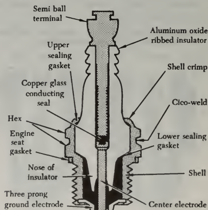
FIGURE 4-25. A typical spark plug.
